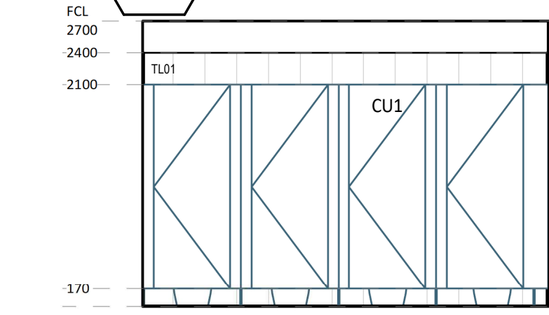
2 ELEVATION DETAIL 1 : 50
