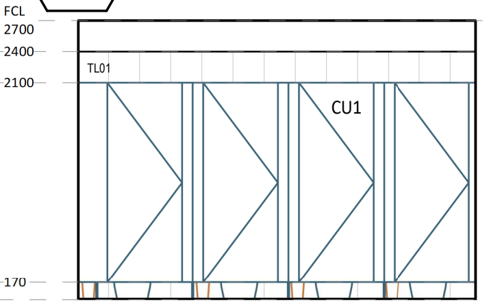
7 ELEVATION DETAIL 1 : 50
