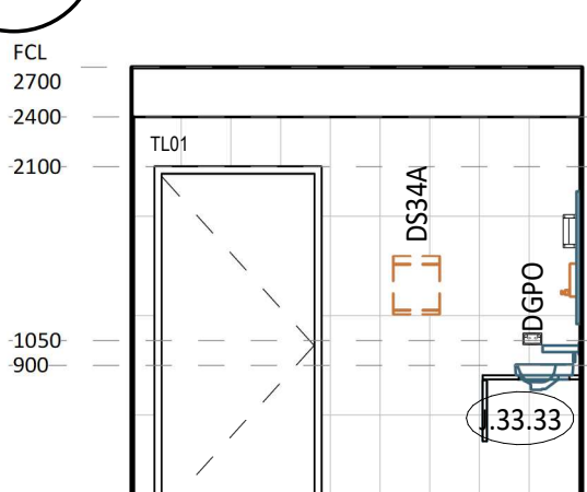
9 ELEVATION DETAIL 1 : 50
